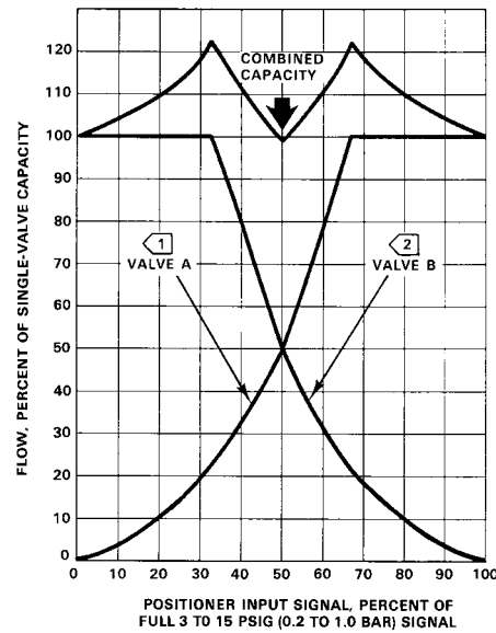
Figure 3. Three-Way Valve Capacity with Dual Actuators--60 Degree Maximum Valve Disc Rotation
