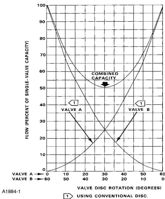
Figure 1. Three-Way Valve Capacity with Single Actuator--60 Degree Maximum Valve Disc Rotation
